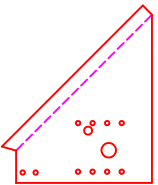
Detail: Stiffener & Jack Mount 1/4" Pl Formed Material 2 Req
