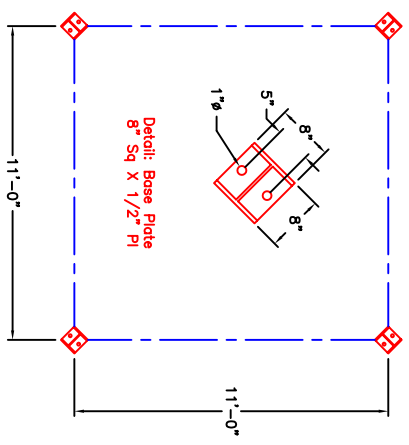
Plan: Base Plate Layout
